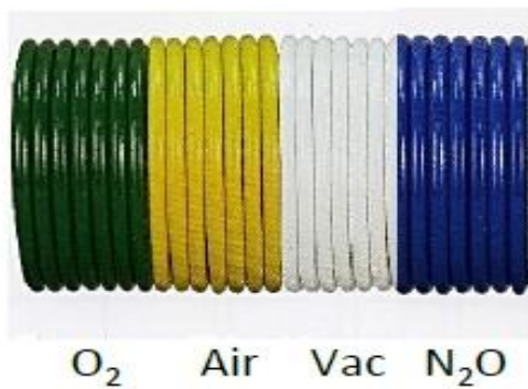
Hose
